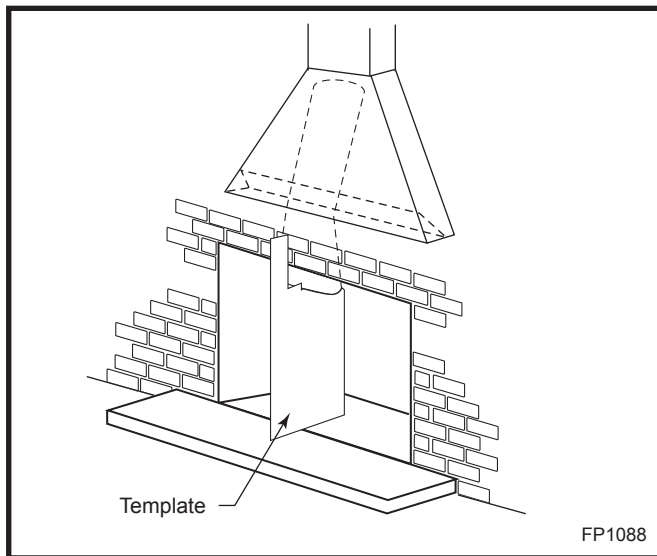
Fig. 23 Using the template that came with the WinterWarm will help you position Flex Connector.
