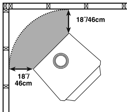
Figure 6 – Top View Minimum Corner Clearances from Combustible Surfaces 18\"/>
