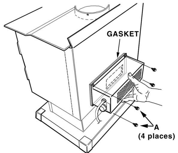
Figure 3 – Attach Optional Blower to Stove Body
